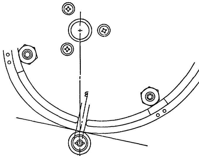
INITIAL CAM POSITIONING RELATIVE TO SOLID PORTION 6-34
