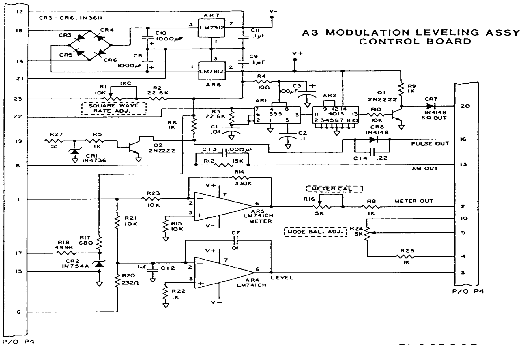
Figure FO-2. Schematic Diagram AN/USM-213B (Sheet 3 of 3)
