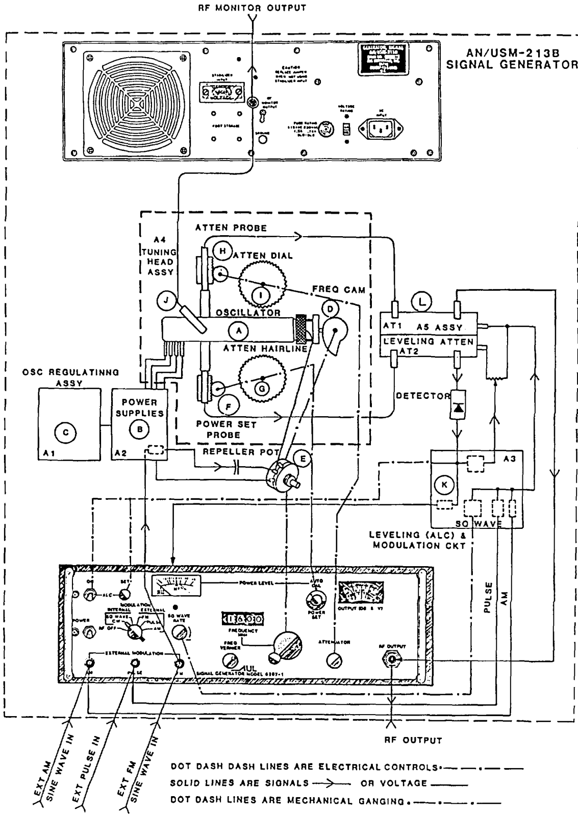
Figure 1-3. Simplified Block Diagram
